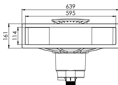
Dimensions for the concrete-liner version
