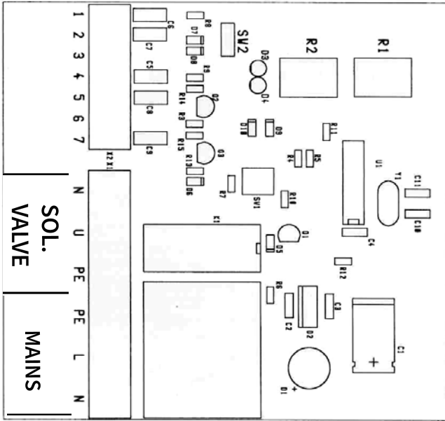
Circuit board.
